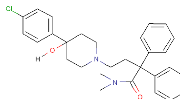
loperamide
