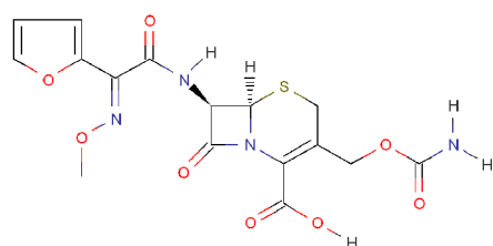
cefuroxime
