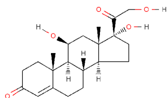
hydrocortisone
