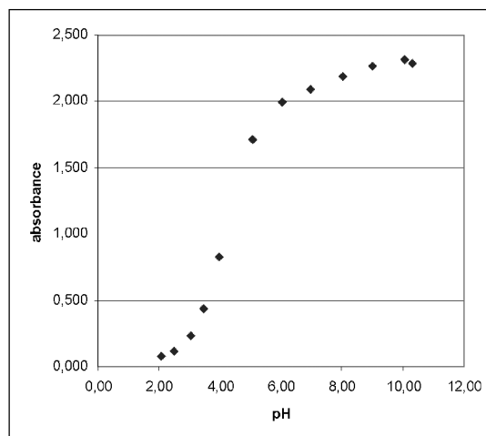
Figure 2. Dependence of absorbance of DTNB degradation products on pH at a wavelength of 415 nm.
