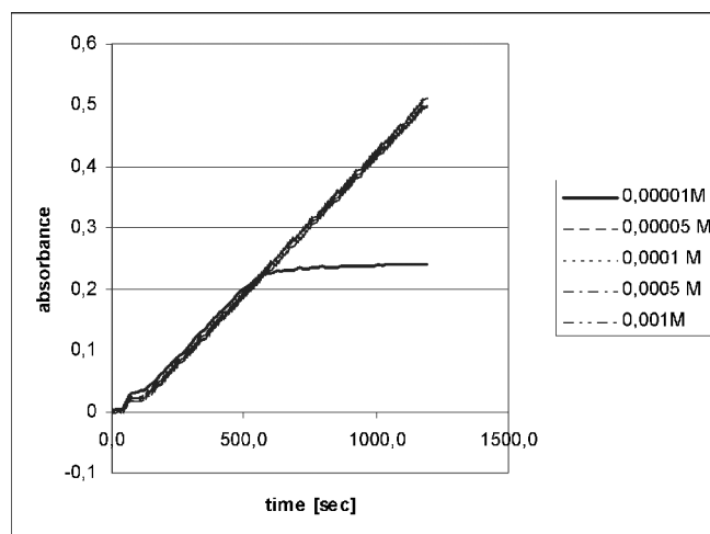
Figure 1. Dependence of absorbance of the reaction mixture in dependence on time and DTNB concentration.
